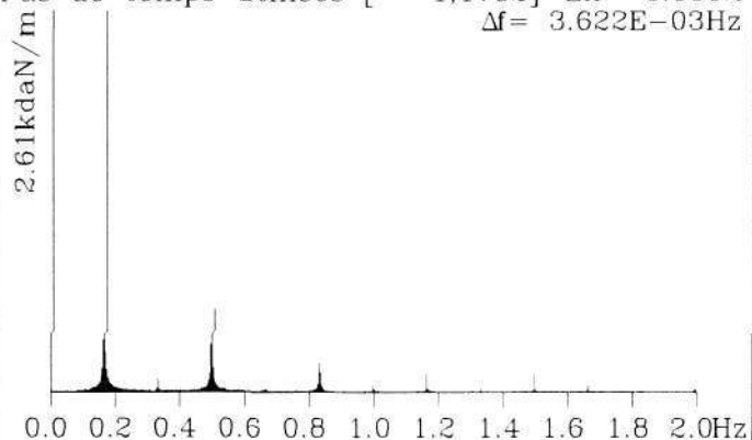
Force resultante / metre
